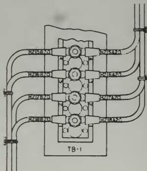
FIGURE 4-87. Wire identification at a terminal block.
